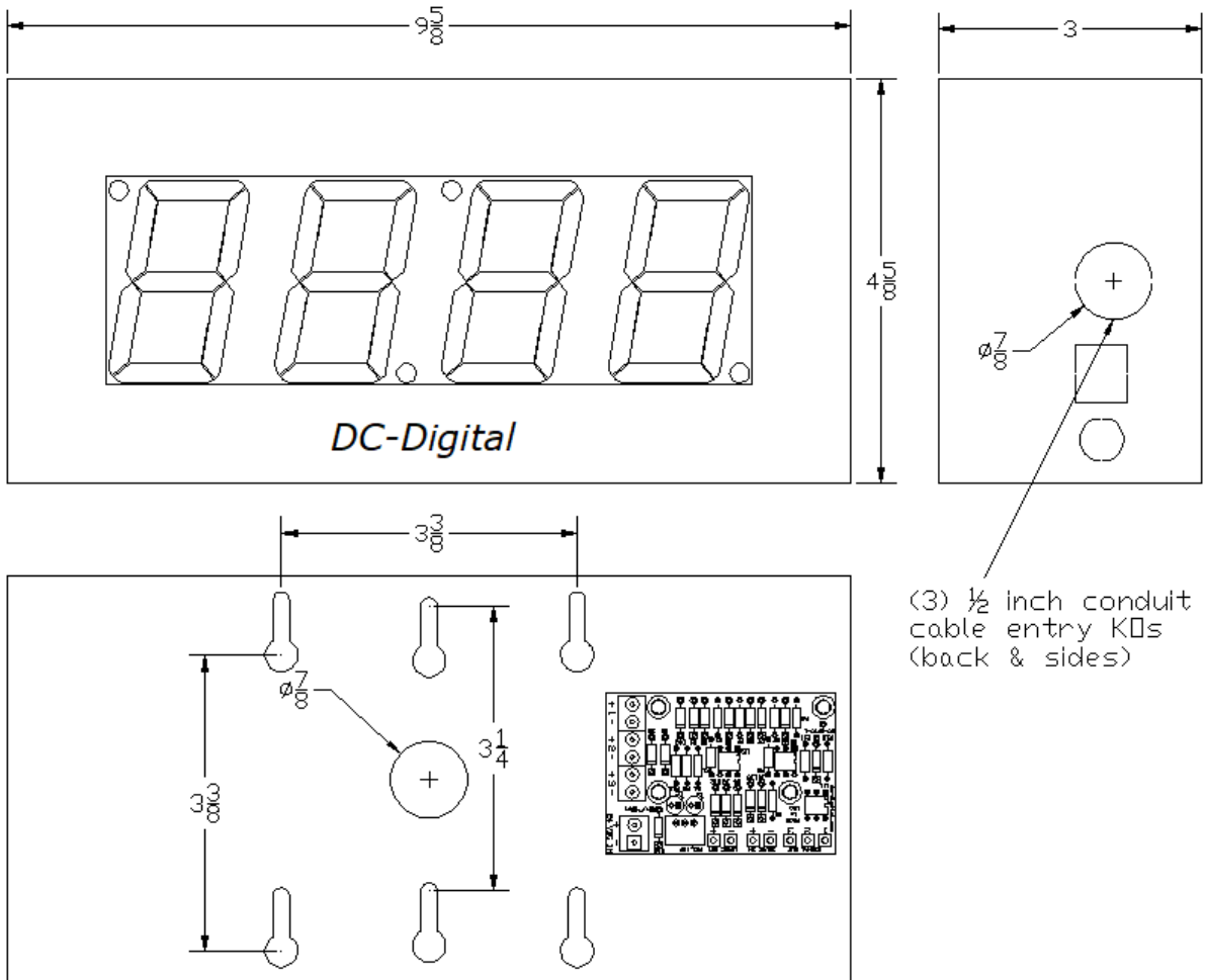
DC-25 Enclosure
