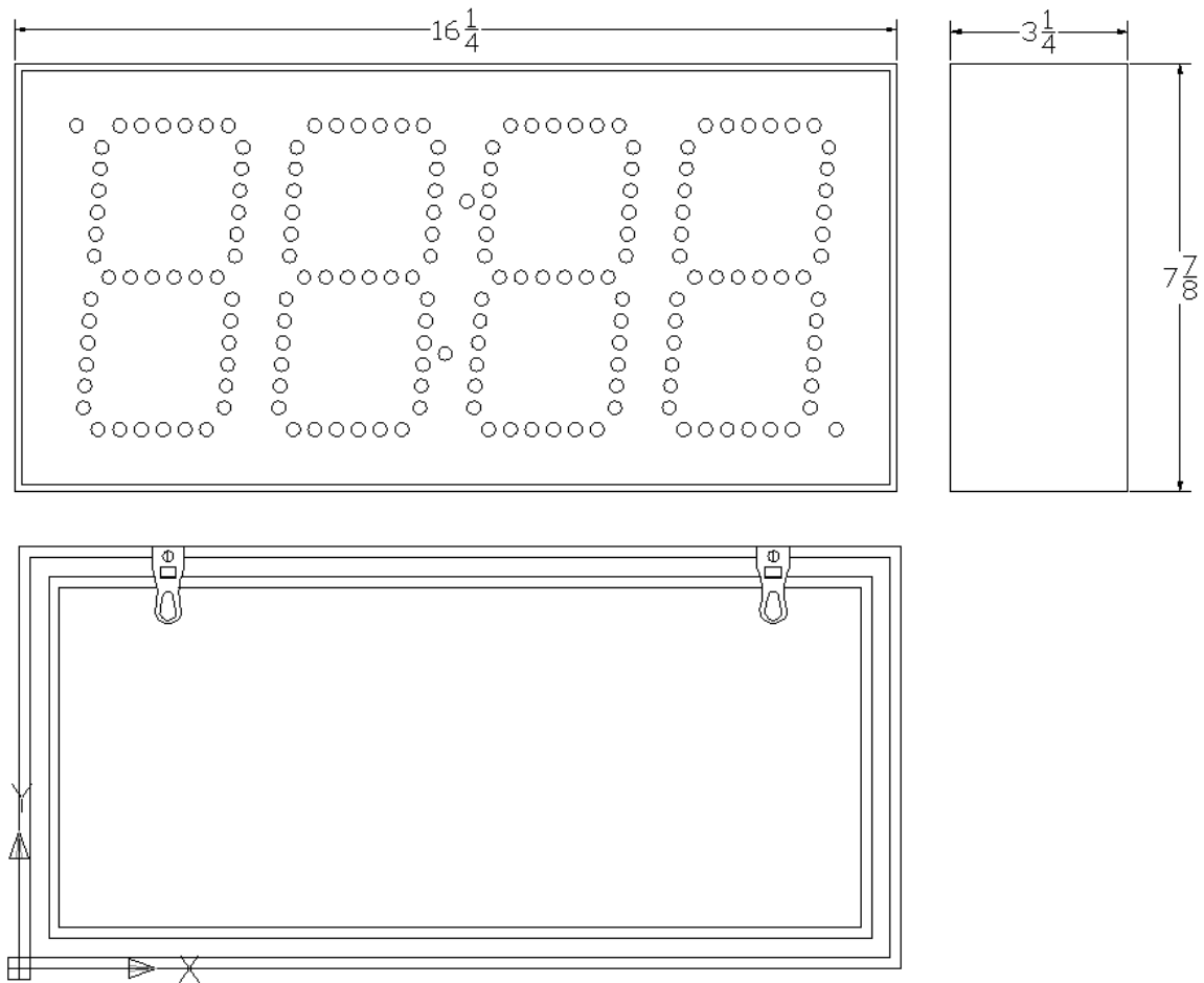
DC-60 Enclosure
