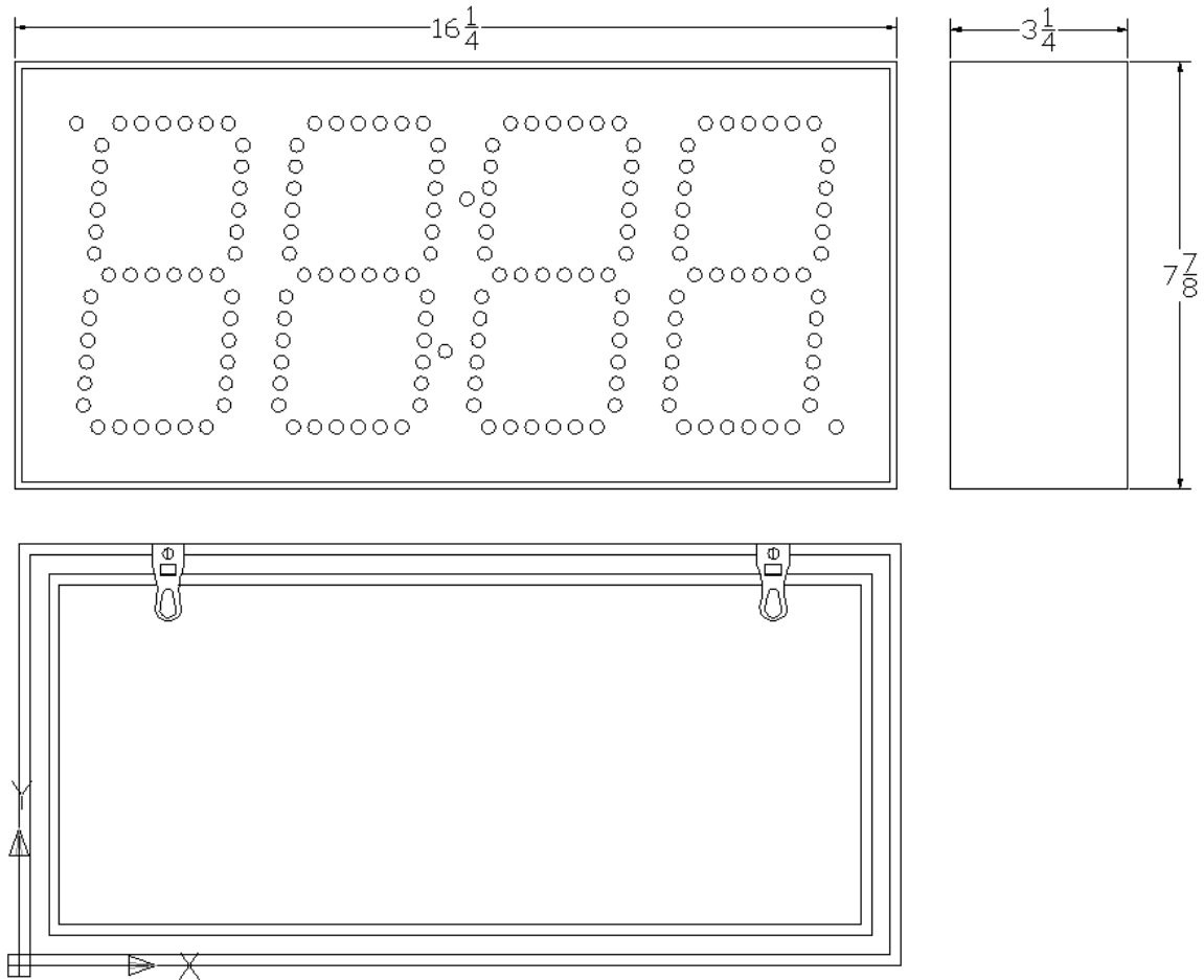
DC-60 Enclosure
