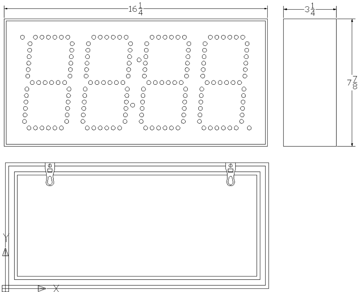
DC-60 Enclosure
