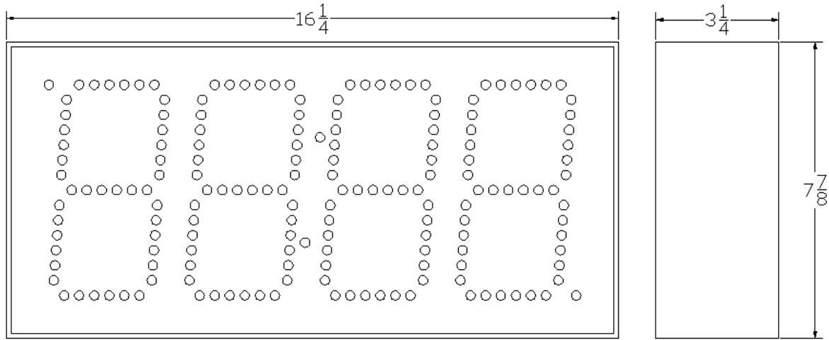
DC-60 Enclosure
